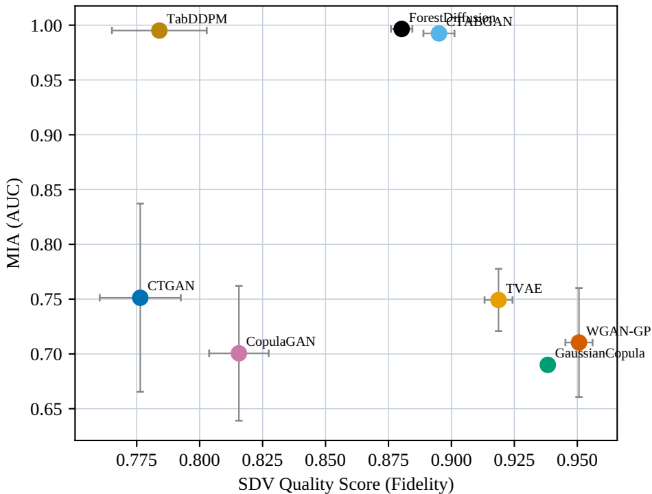
Wine Quality: SDV Quality Score (Fidelity) vs MIA (AUC)
